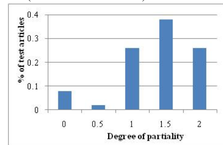
Figure 2. Distribution of degrees of partiality
