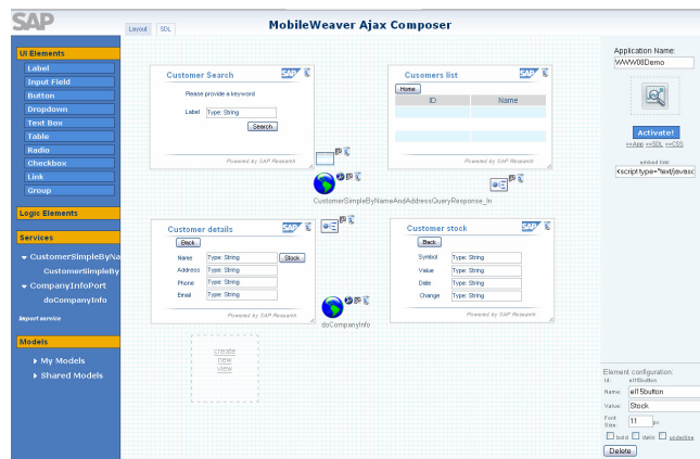
Figure 2. MobileWeaver Ajax Composer.
