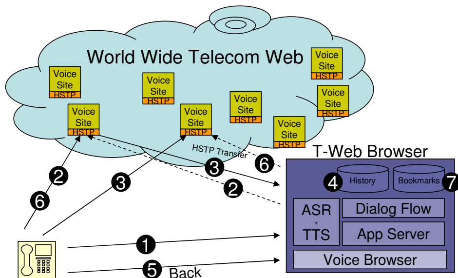
Figure 2: The T-Web Browser interaction with VoiceSites.
