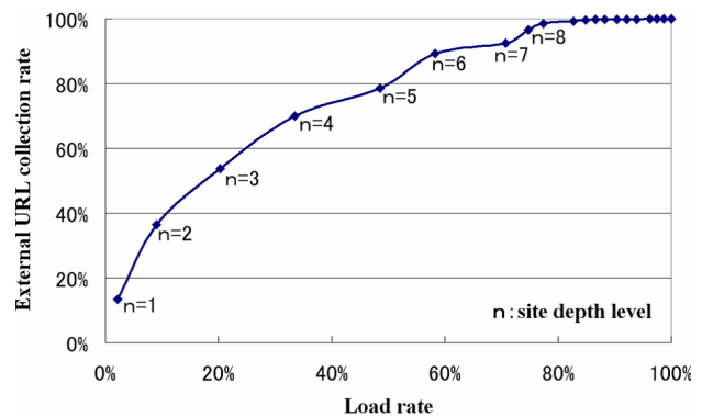
Figure 3: Relation between external URL collection rate and load rate
