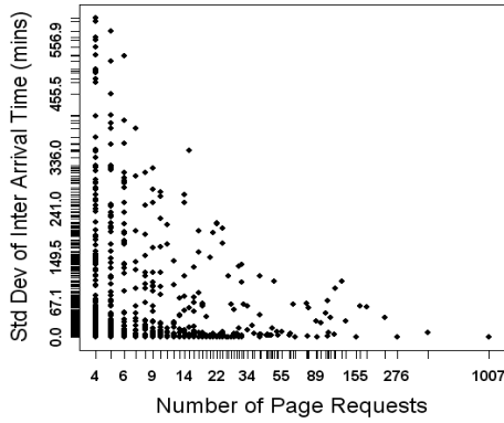
Figure 4: Standard deviation of the inter arrival times (of page requests) for the Page Requesters. The y-axis is plotted on a log scale.
