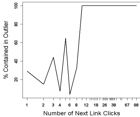
Figure 5: Next Clickers contained in the outliers.
