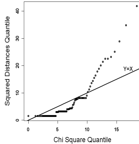
Figure 2: Quantile-Quantile plot of the squared Mahalanobis distance computed from the clickstream data and the \chi_7^2 distribution.
