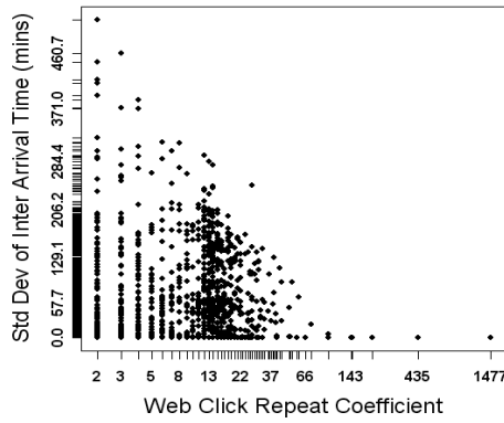
Figure 8: Standard deviation of the inter arrival times (of web results clicks) for the Repeated Web Result Clickers. The y-axis is plotted on a log scale.
