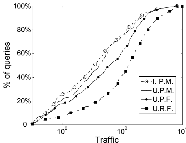
Figure 7. Traffic for distributed intersection using intersection size estimation.
